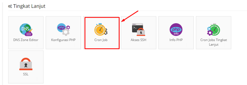
Gambar 5.9. Cron Job
