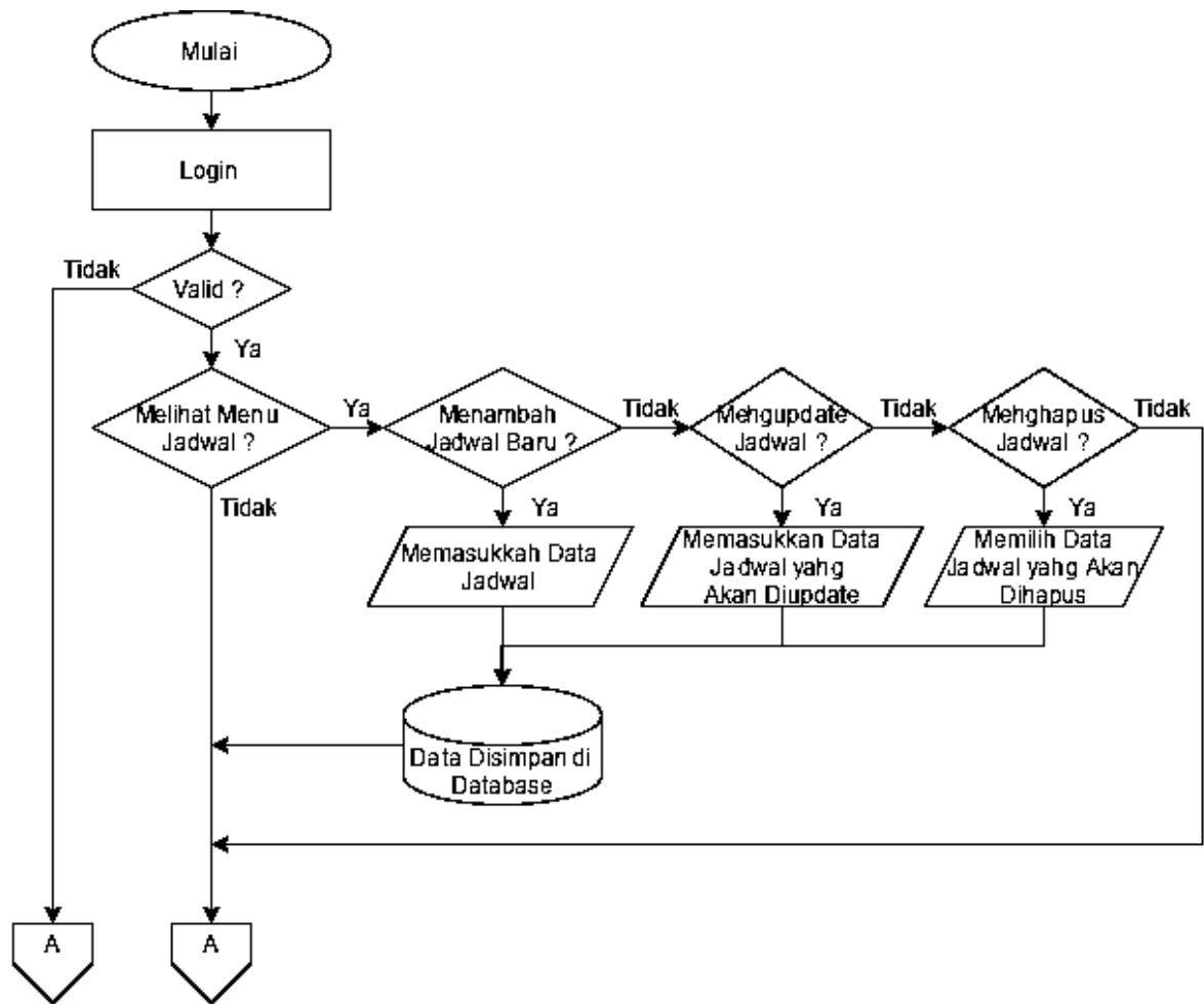
Gambar 1 Flowchart Mentor
