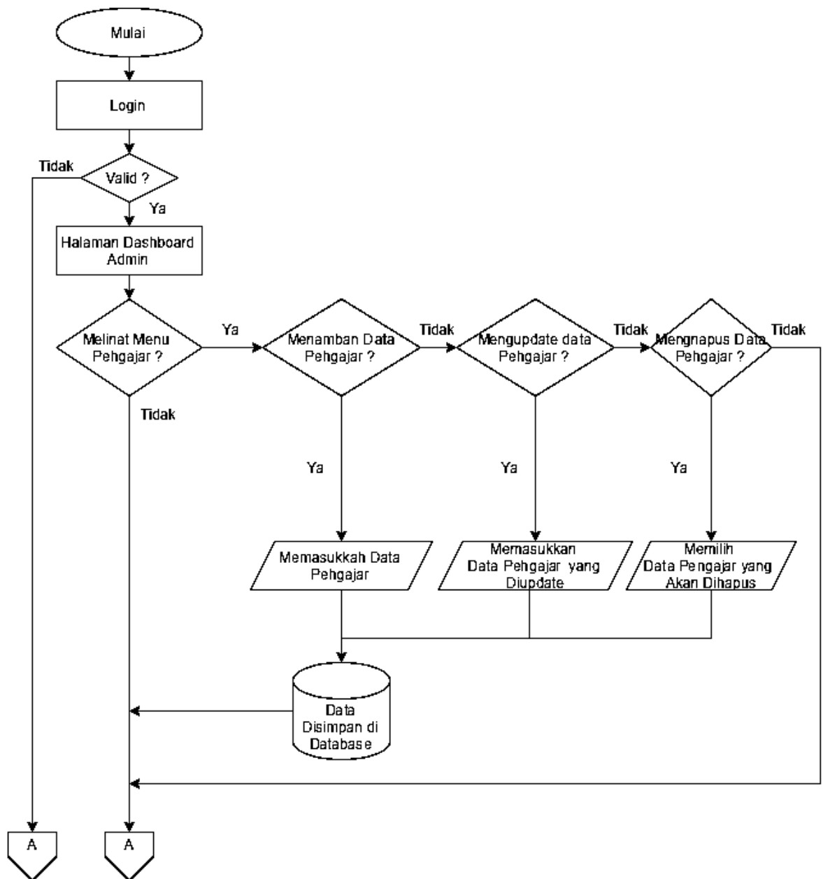
Gambar 1 Flowchart Admin
