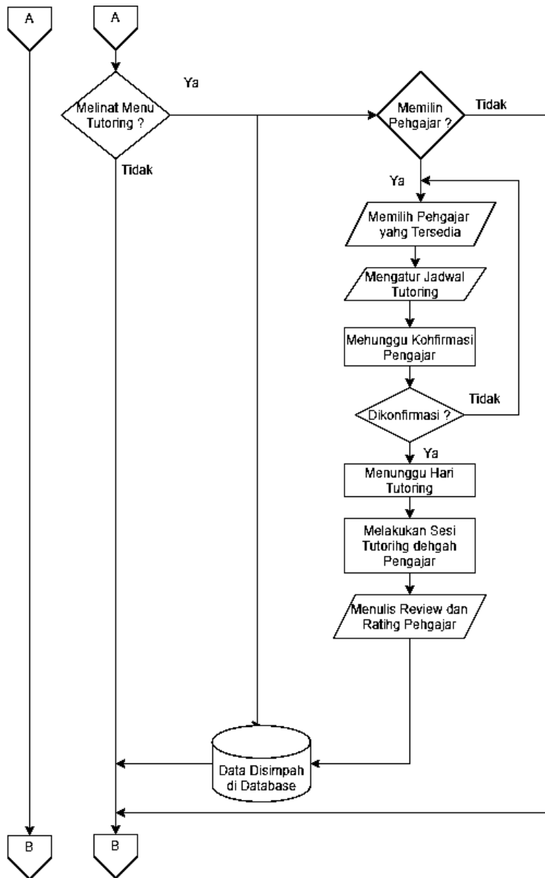
Gambar 2 Flowchart Student
