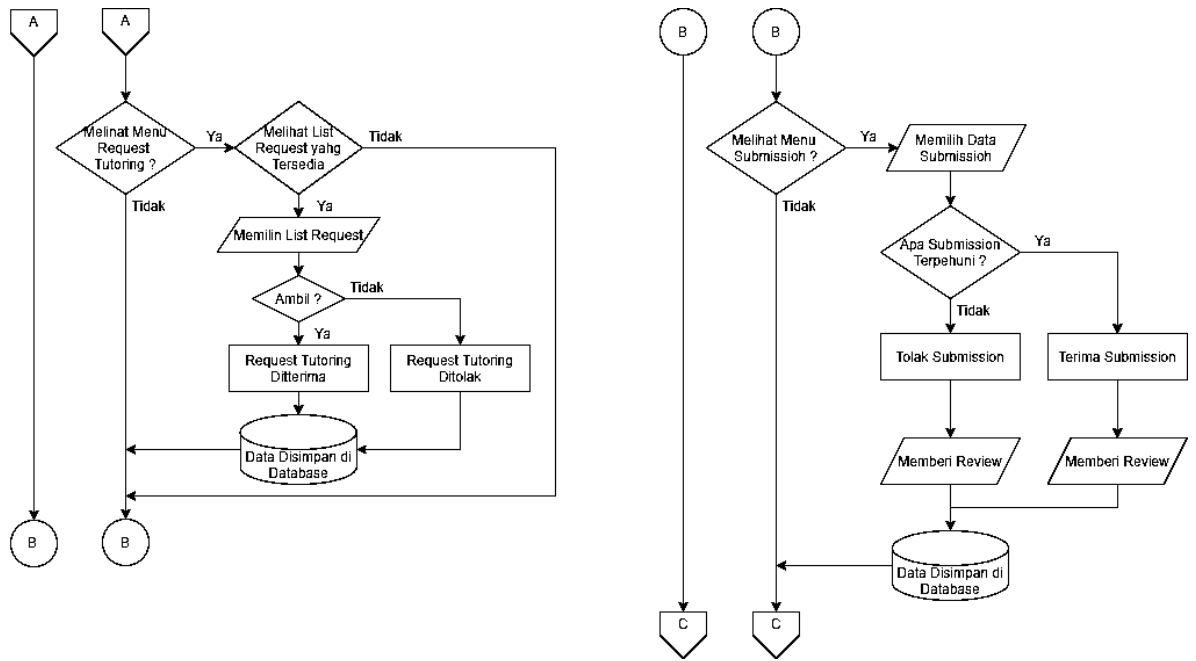
Gambar 2 Flowchart Mentor
