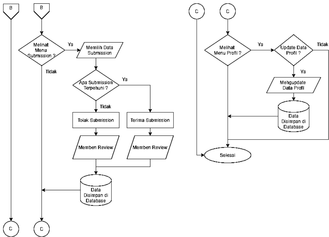
Gambar 3 Flowchart Admin
