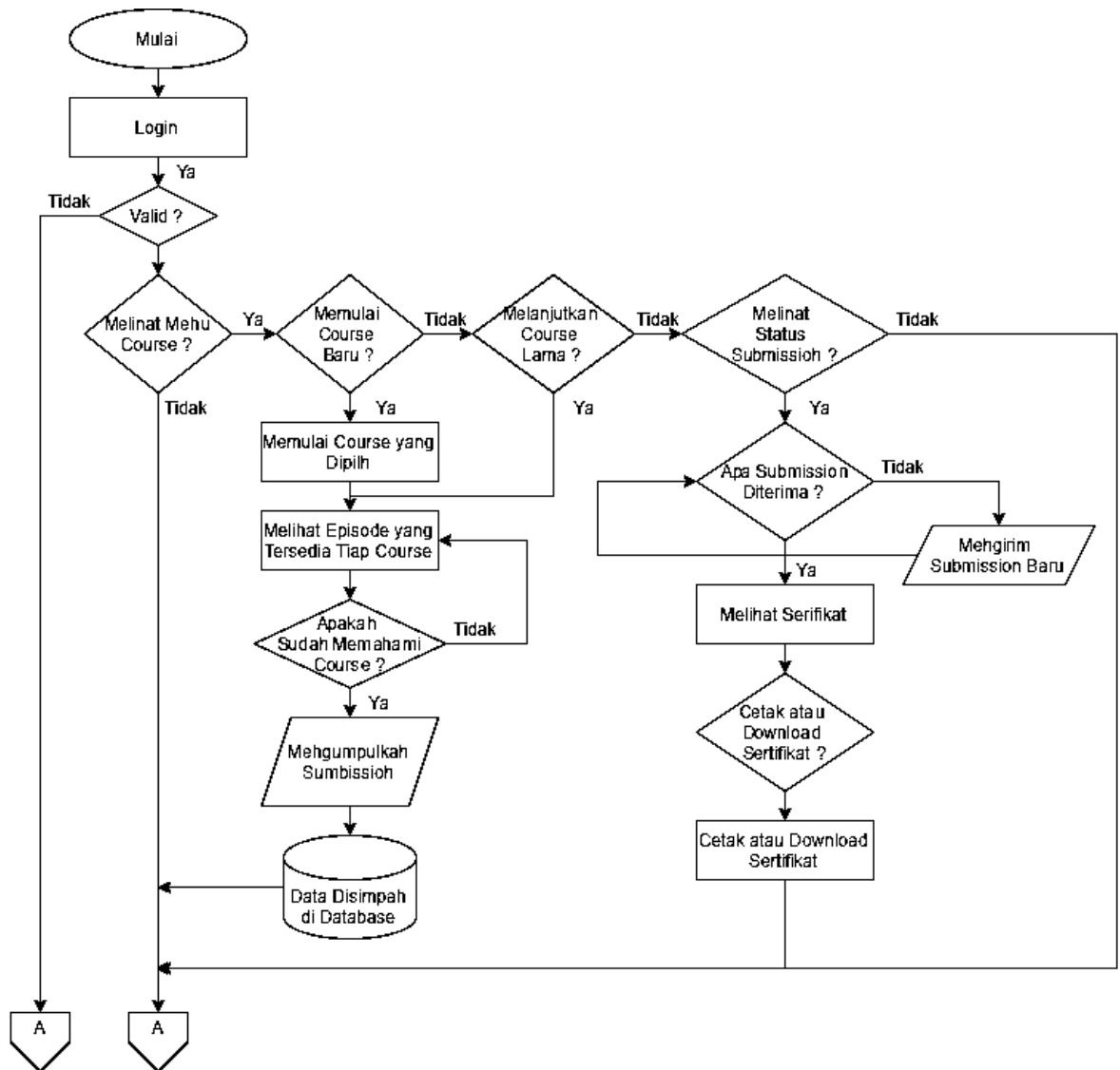
Gambar 1 Flowchart Student
