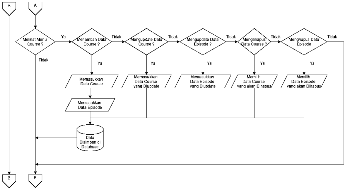
Gambar 2 Flowchart Admin
