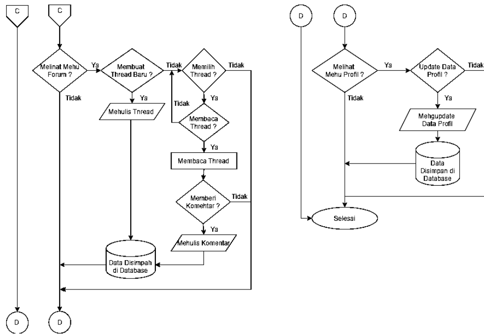
Gambar 3 Flowchart Mentor
