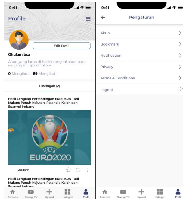
Gambar 5. 12 Purwarupa Halaman Setting
